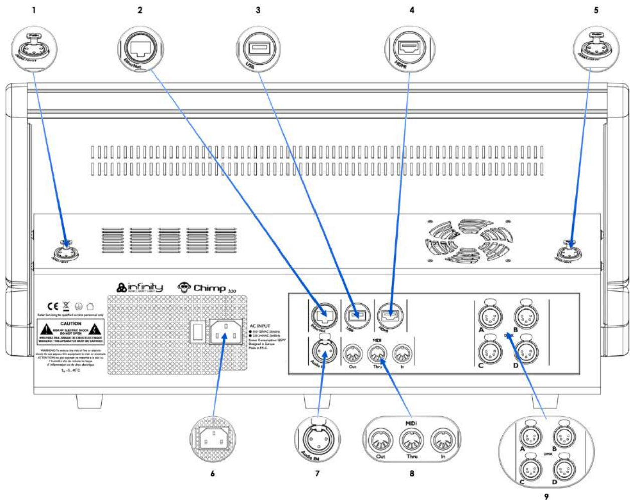
Fig. 2: Chimp 300 Backpanel
