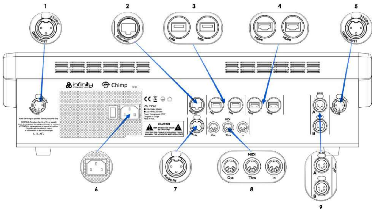
Fig. 1 Chimp 100 Backpanel
